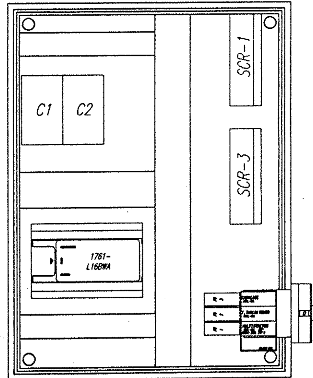
HL66-10 PANEL LAYOUT 16 x 12 x 06
